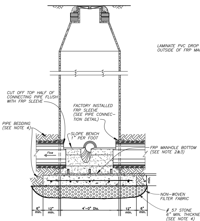
SECTION B-B
